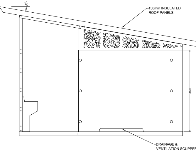
SIDE ELEVATION
